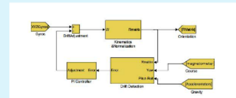
Software
